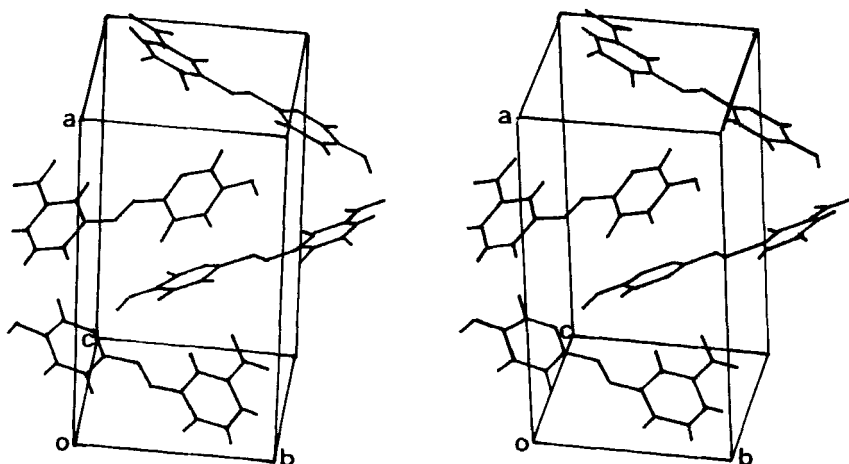
FIGURE 2 Stereodrawing of the crystal packing of the title compound down [001].
