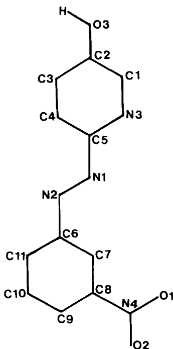
FIGURE 1 Atom—labelling scheme for the title compound.
